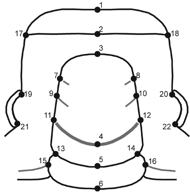
Figure 5: Landmark scheme showing the 22 landmarks used in the morphometric analysis of Prosaukia and Thailandium .
